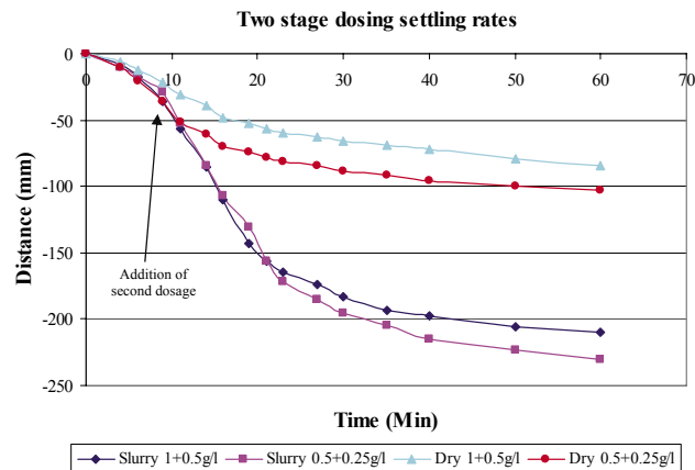
Figure 4 Two-stage dosing settling rates (compare with Fig. 5 where different 1:0.5 ratios were evaluated)
