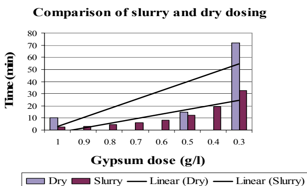
Figure 3 Comparison between slurry and dry dosing settling rates
